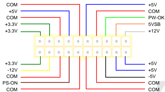
Power Connector
