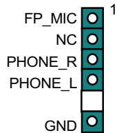
AUDIO1 Connector
