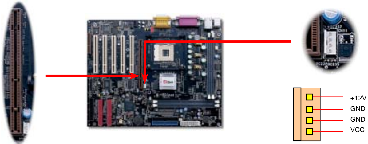
AGP Pro Expansion Slot
