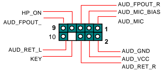
AUDIO Connector
