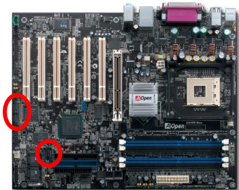
SATA 連接埠 1 (ICH5R)
