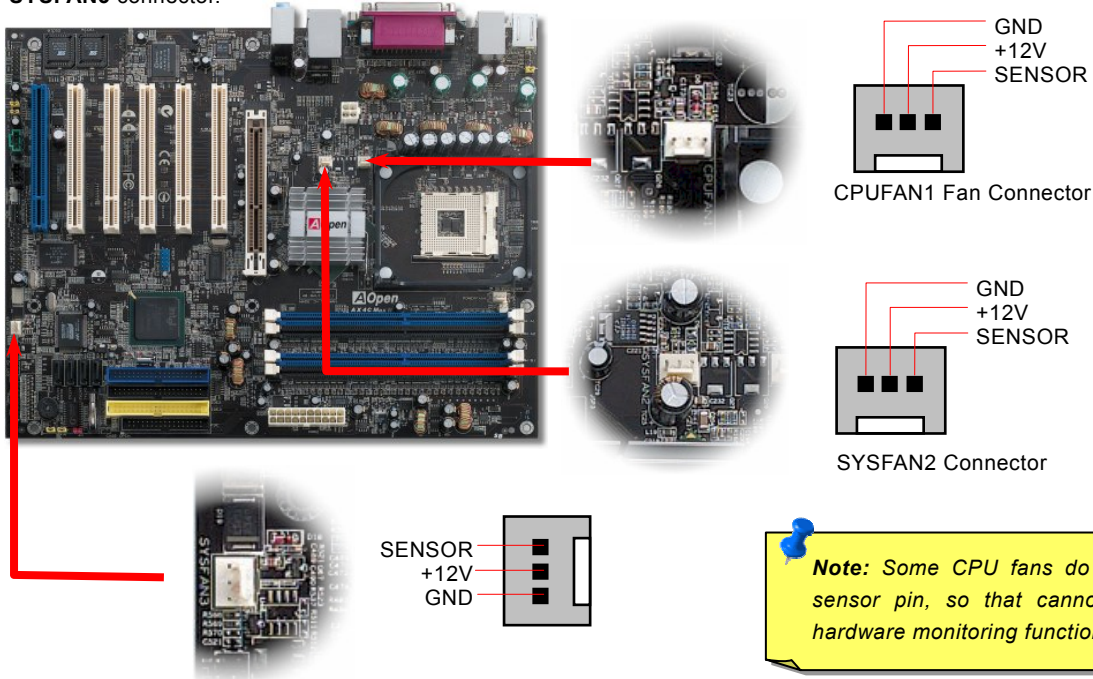
SYSFAN3 Connector
