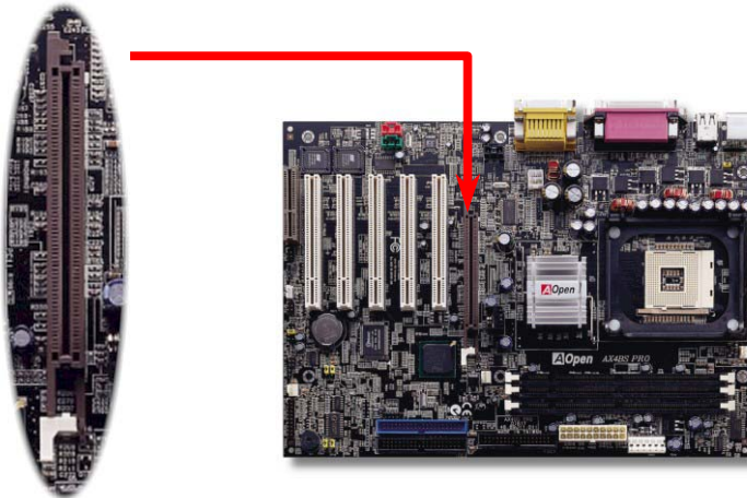
AGP Expansion Slot
