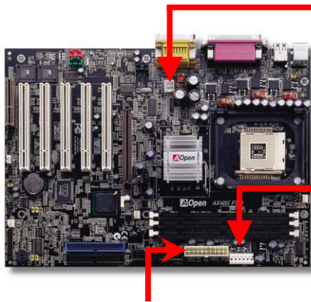
Extra Power Connector for 5V/3.3V
