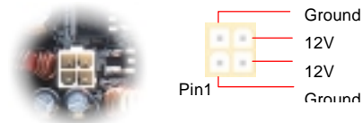
4-Pin 12V ATX Power Connector
