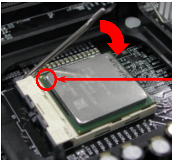
Bisel CPU
