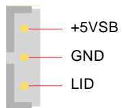
Conector WOL
