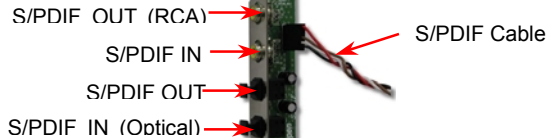
S/PDIF Module (User Upgrade Optional)
