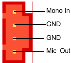
MODEM-CN
