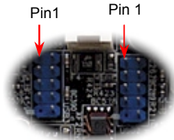
USB2.0 Connector
