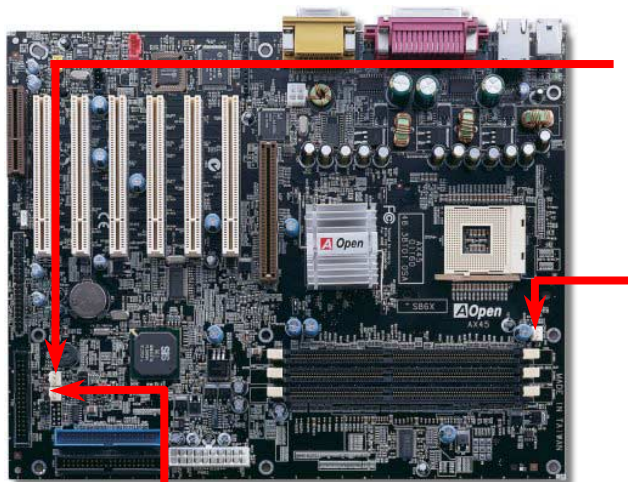
FAN3 Connector
