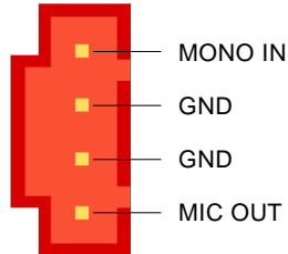
MODEM-CN Connector
