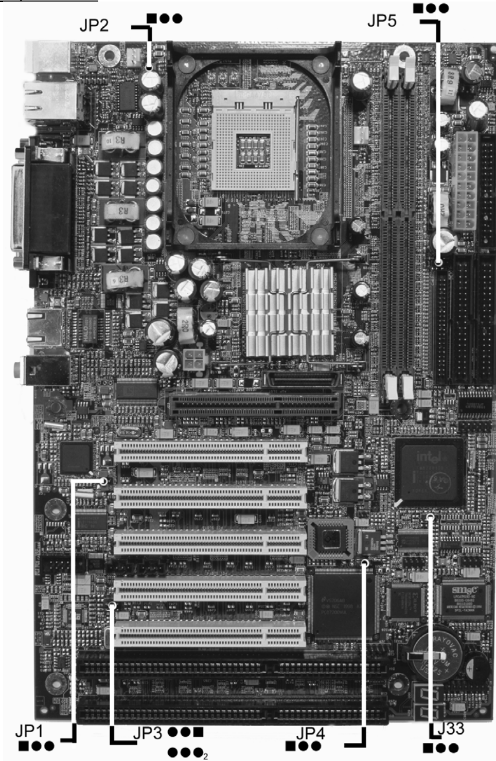
Figure 1-1 Jumper Locations
