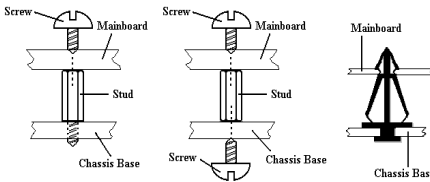
Figure 2-4. The way we fixed the motherboard
