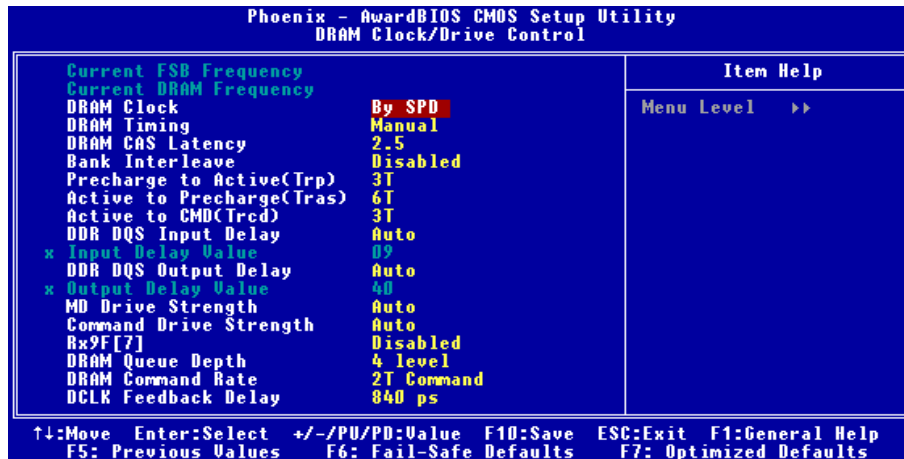
Figure 3-5B. DRAM Clock/Drive Control Screen
