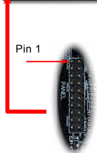
Front Panel Connector
