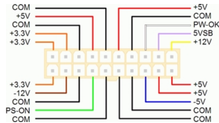
20-Pin Power Connector
