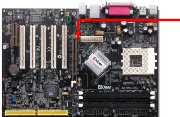
AGP LED
