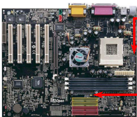
SW1 CPU Ratio Select Switch
