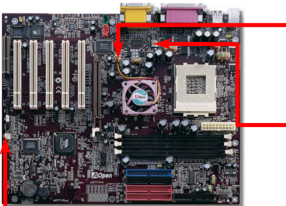
GND +12V SENSOR
