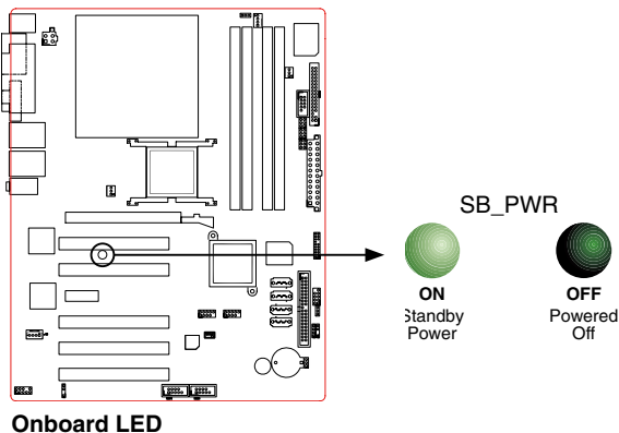
Onboard LED
