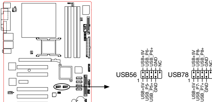
USB 2.0 connectors
