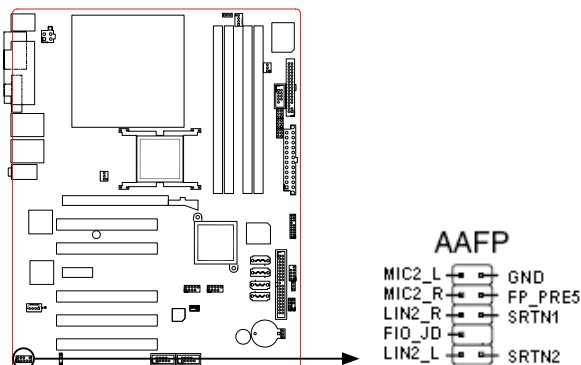
Analog front panel connector
