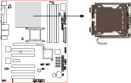
CPU Socket 775
