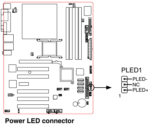
Power LED connector
