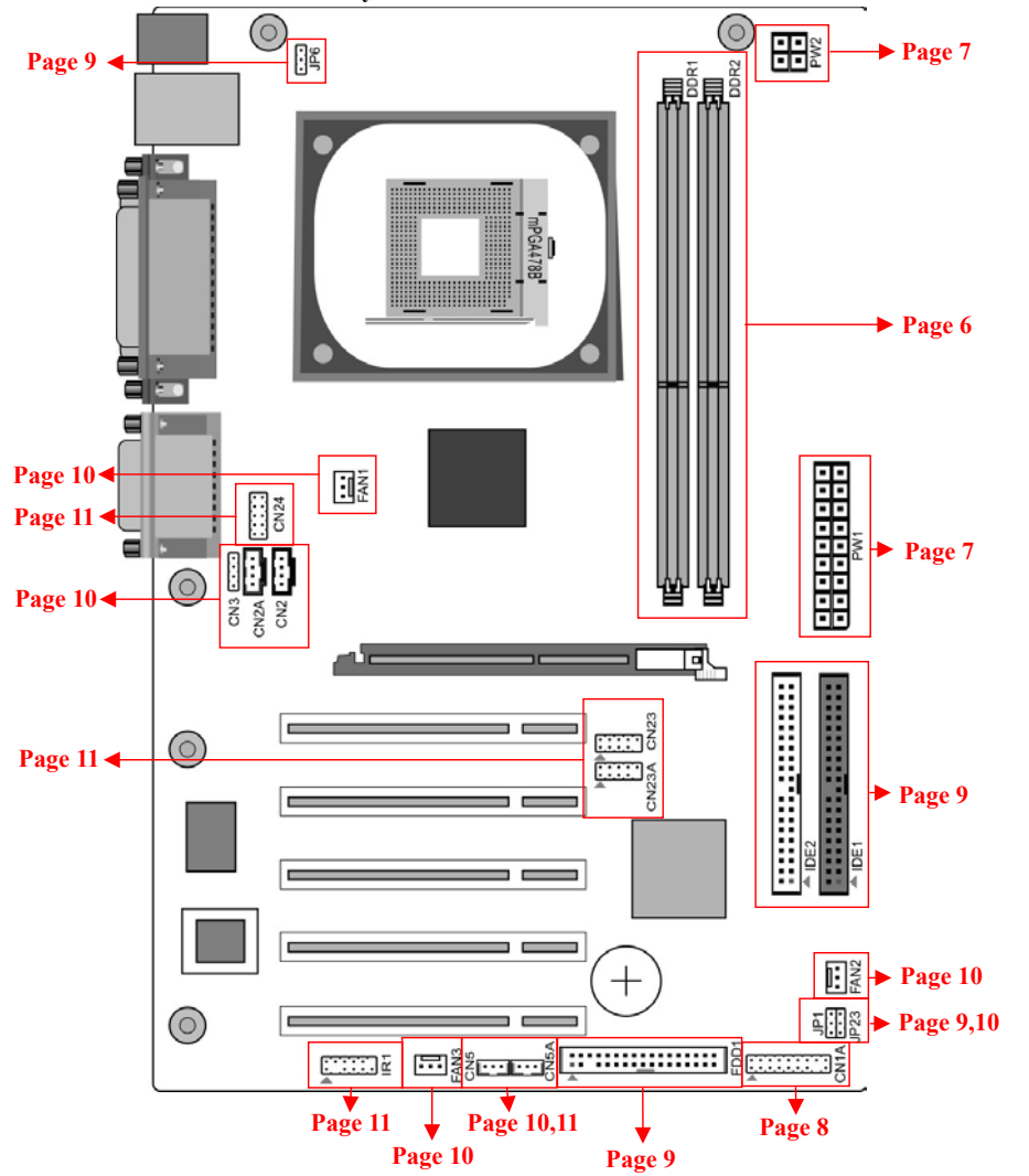
1-4 9VJL3 Motherboard Layout
