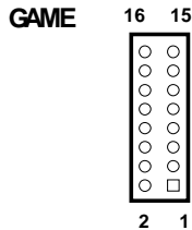
GAME PORT Connector
