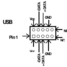
USB Port Connector
