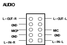
Audio Connector
