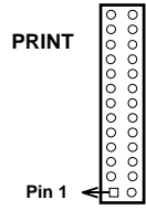
Parallel Printer Connector
