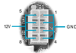
8-pin ATX_12 V Power Connector
