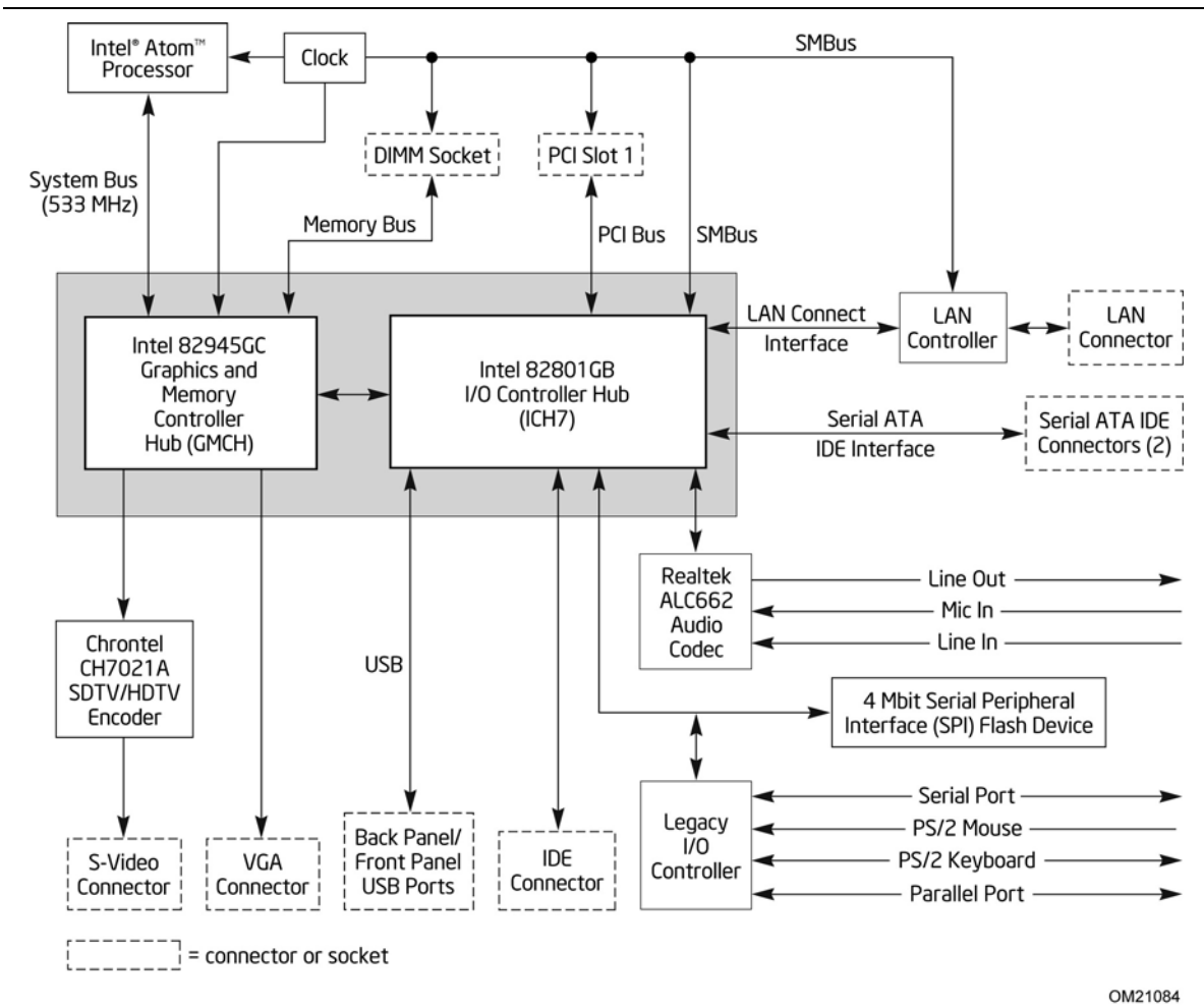
Figure 2. Block Diagram
