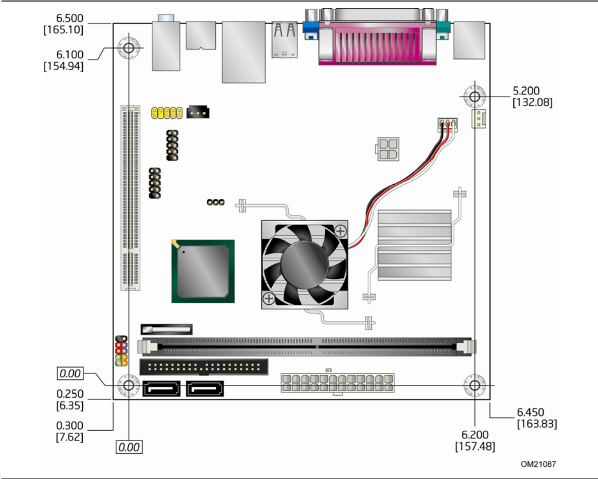
Figure 13. Board Dimensions
