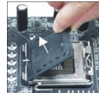
Yellow triangle is the Pin 1 indicator
