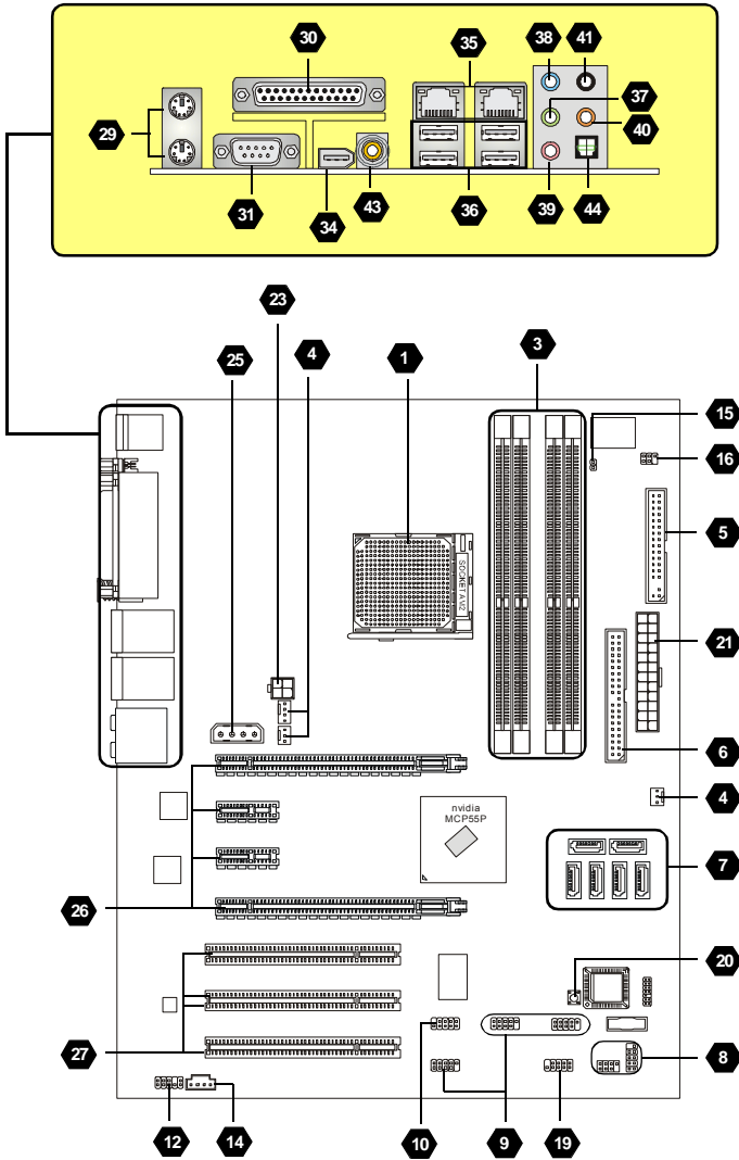
Layout of K9N SLI Platinum Series (MS-7250 v1.X) Mainboard
