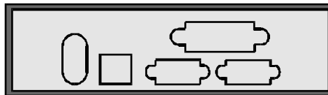
Figure 1-3 Mini-ATX I/O shield
