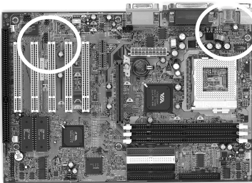
USB 2/3 USB 0/1 ports
