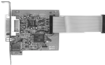
Figure 1-3 LTI-II Header
