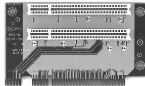
Figure 1-4 PCI Riser card
