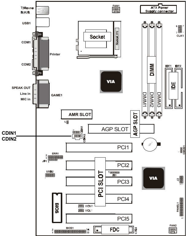
1.9.1 CD Audio-In Connectors:CDIN1/CDIN2
