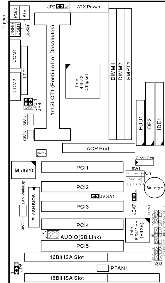
Figure 1-1. Motherboard Layout
