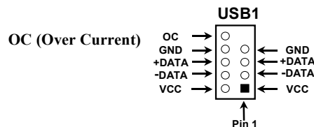
USB Port Headers
