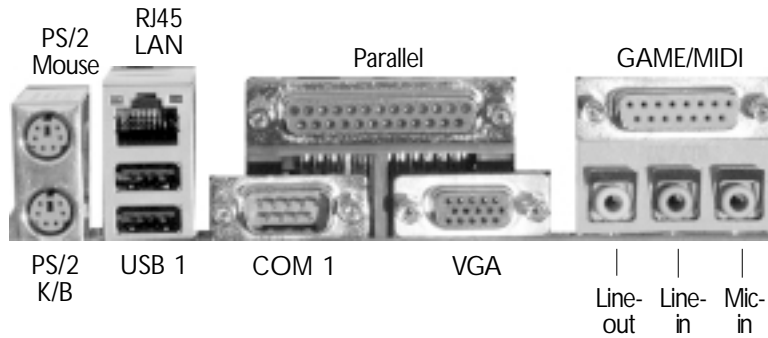
ATX Double Deck Ports on NB76-TL
