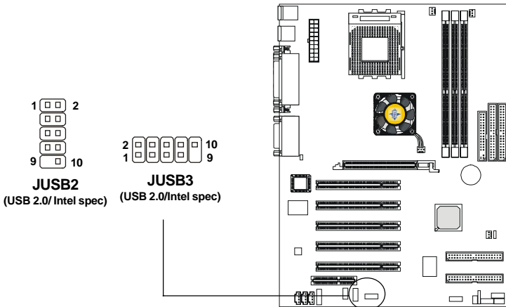
JUSB2/3 Pin Definition
