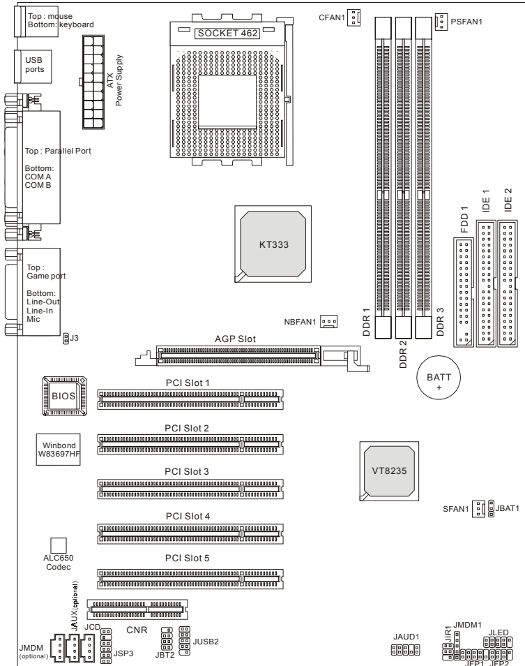
KT3 Ultra2 (MS-6380E) ATX Mainboard
