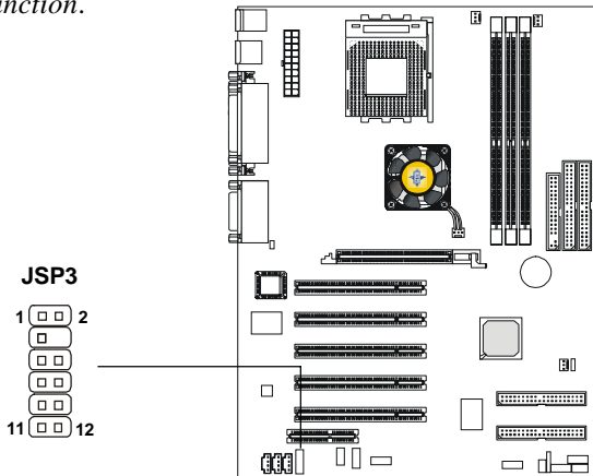
JSP3 Pin Definition
