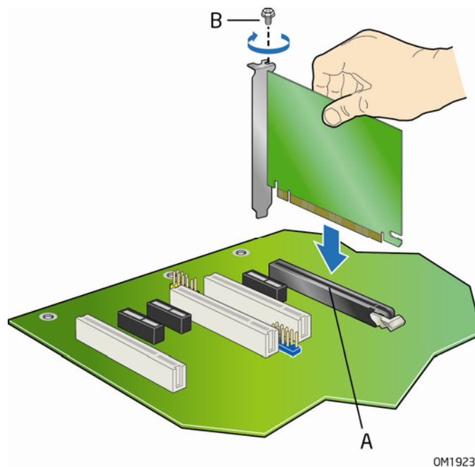
Figure 18. Installing a PCI Express x16 Card
