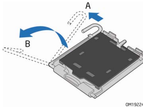
Figure 6. Lift Socket Lever
