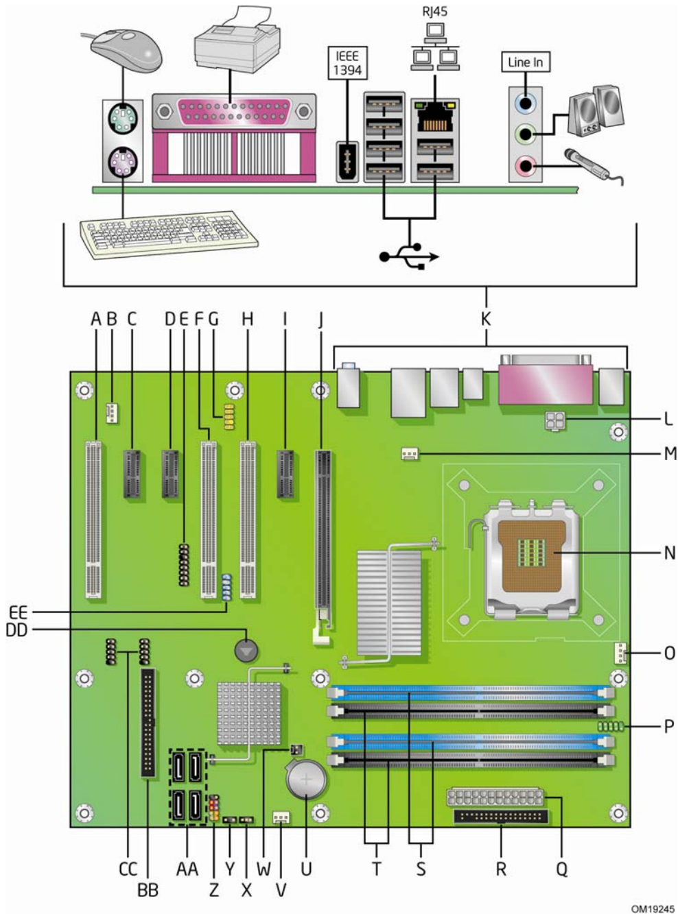
Figure 1. Desktop Board DP965LT Components
