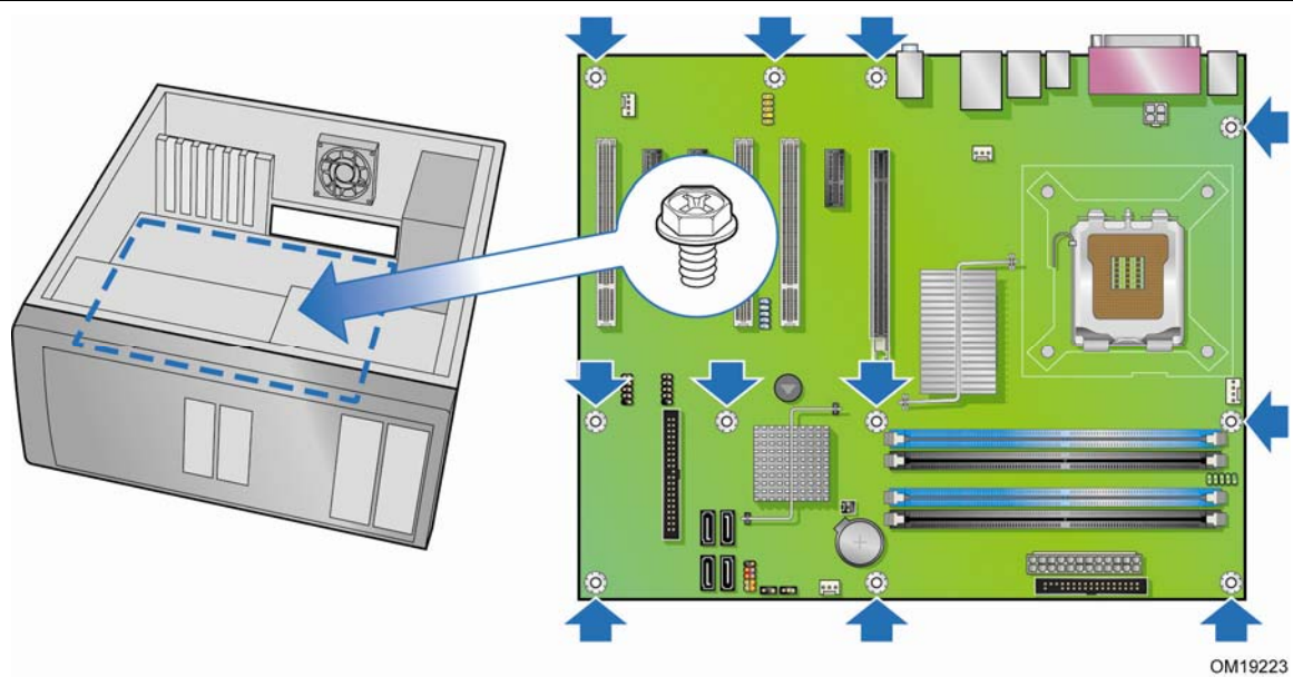
Figure 5. Desktop Board DP965LT Mounting Screw Hole Locations
