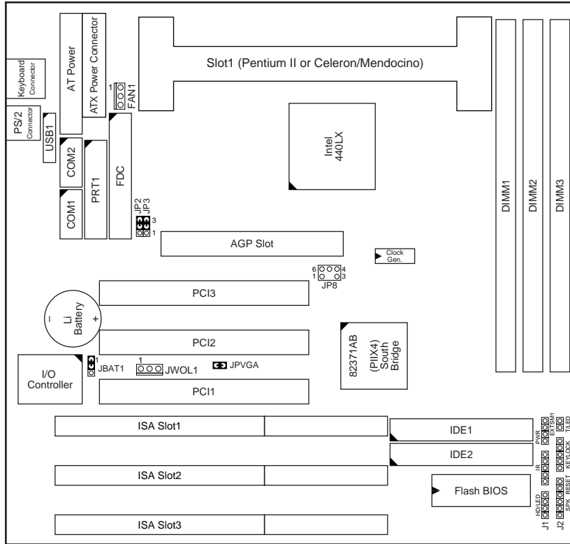
Figure 1-1. Motherboard Layout
