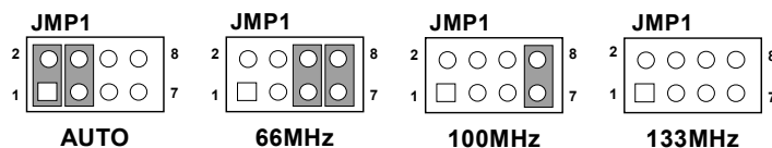
CPU F.S.B. Clock Setting
