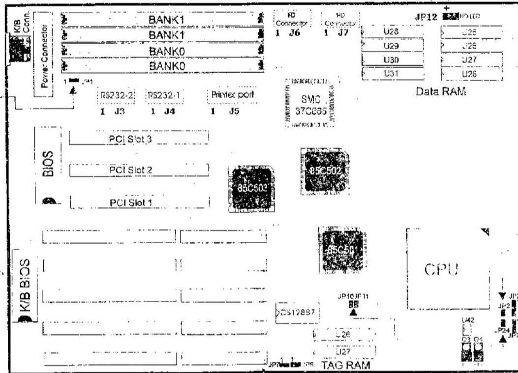
JP7,JP8 : Cache Size Selector Jumper
