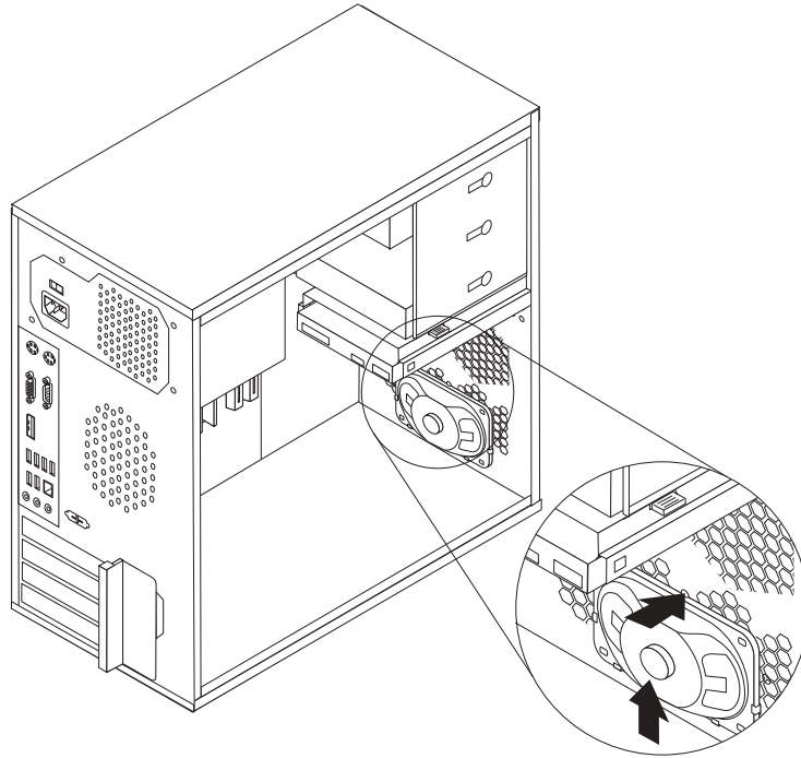
Figure 34. Removing the old internal speaker
