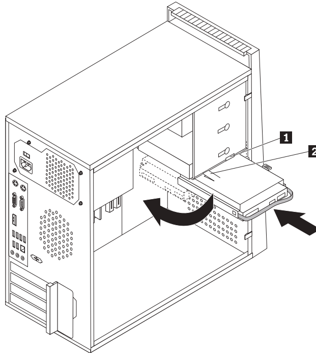
Figure 22. Installing the primary hard disk drive with the hard disk drive cage
