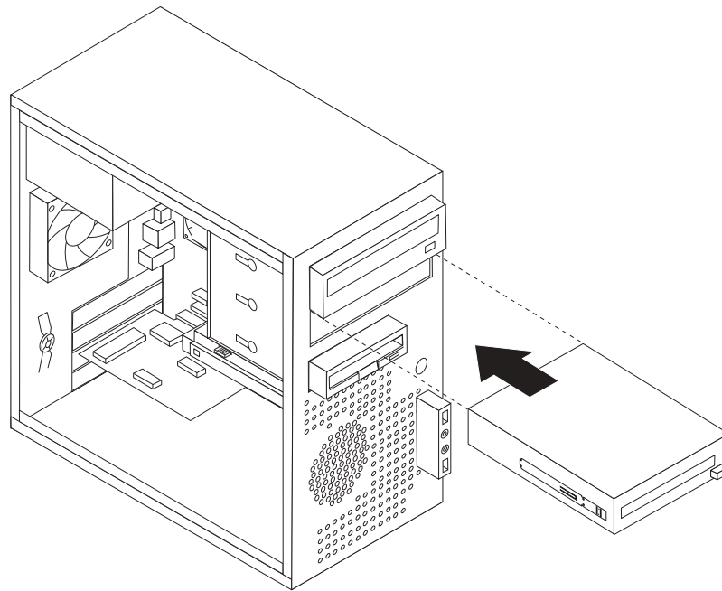
Figure 14. Installing the drive
