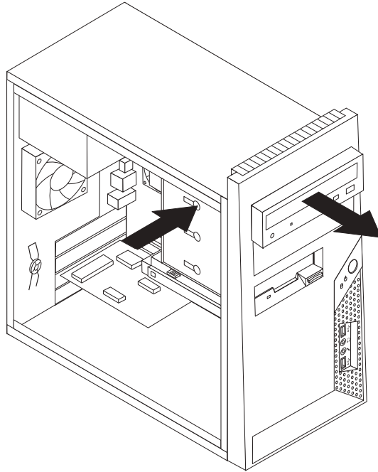
Figure 26. Removing the optical drive
