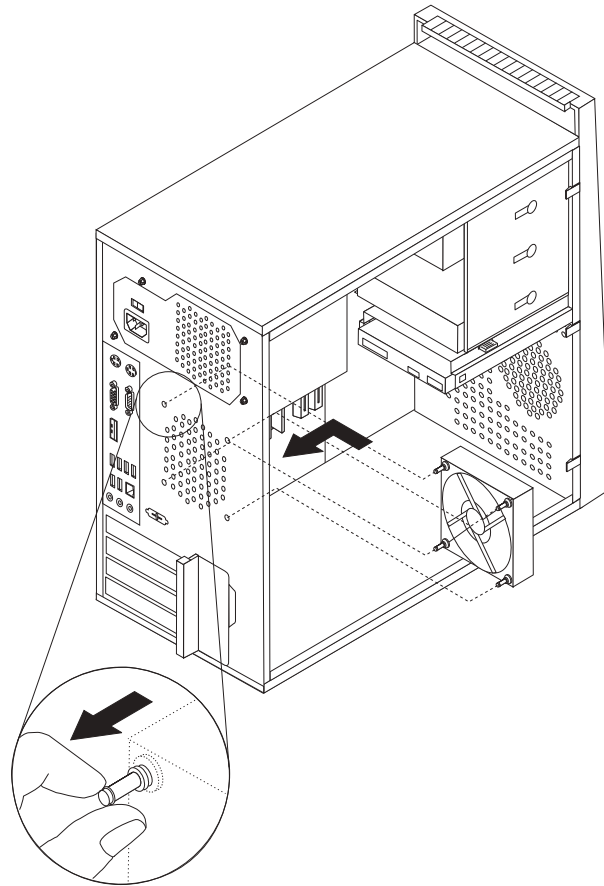
Figure 33. Installing the rear fan assembly
