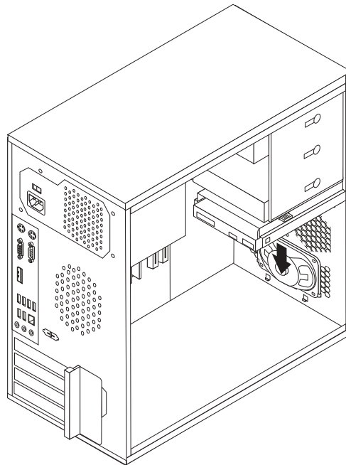
Figure 35. Installing a new internal speaker
