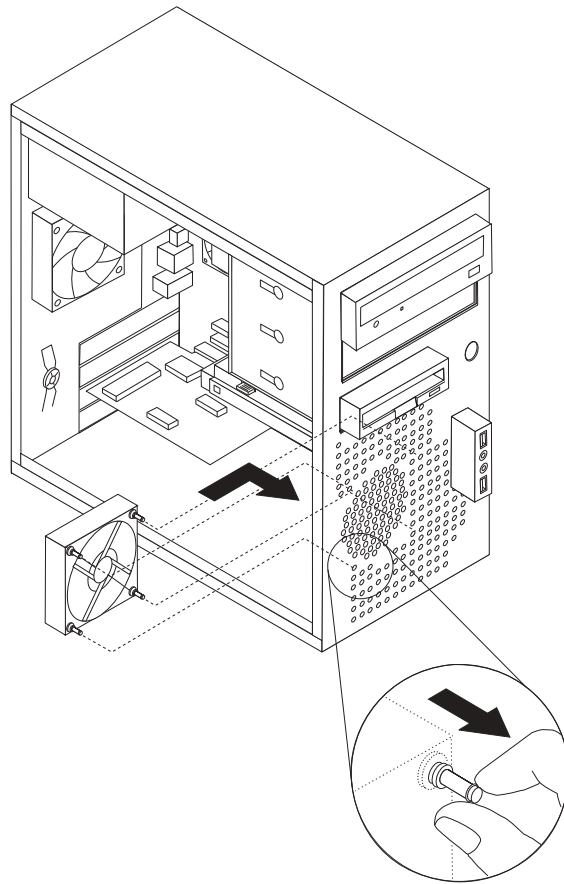
Figure 31. Installing the front fan assembly
