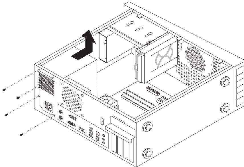
Figure 18. Removing the retaining screws for the power supply assembly
