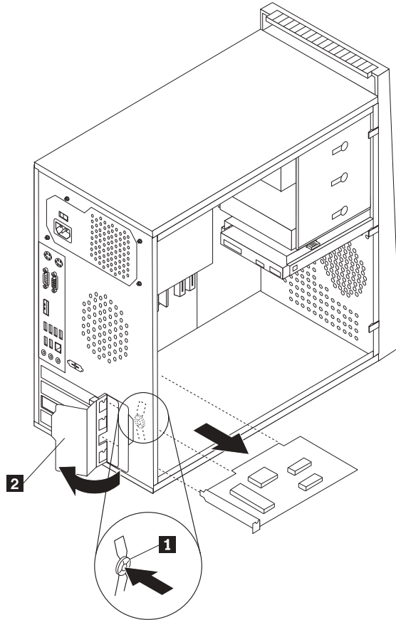
Figure 7. Opening the card latch
