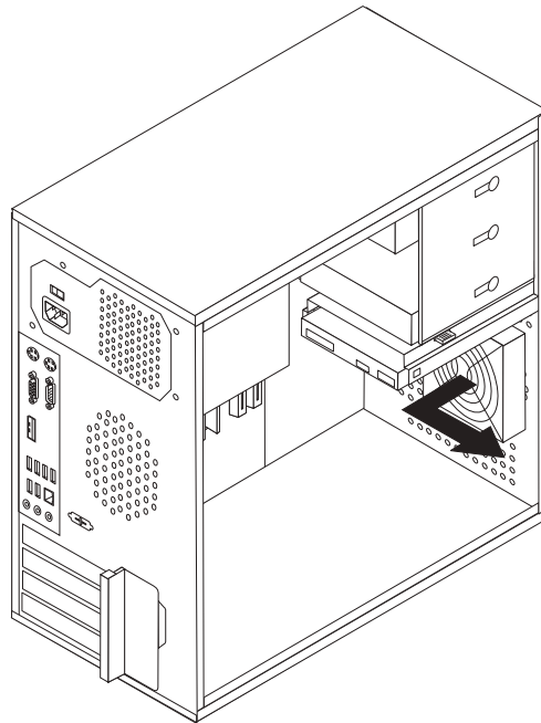
Figure 30. Removing the front fan assembly
