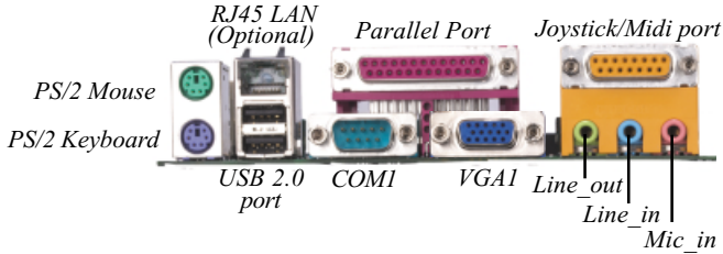
Figure 11 - I/O Ports
