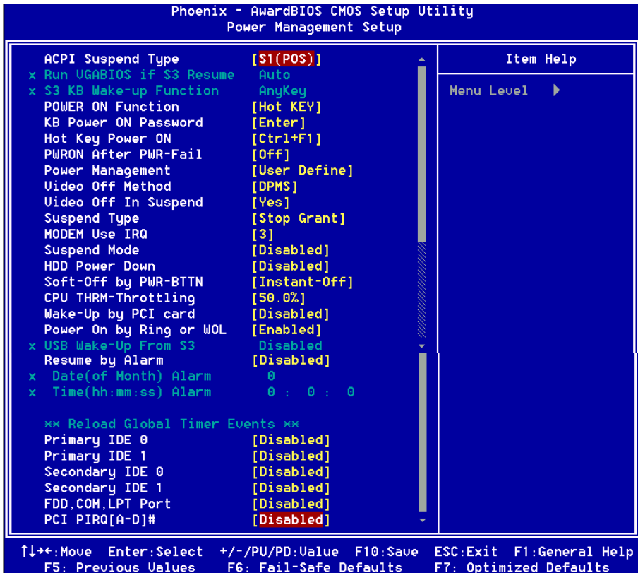
Figure 6: Power Management
