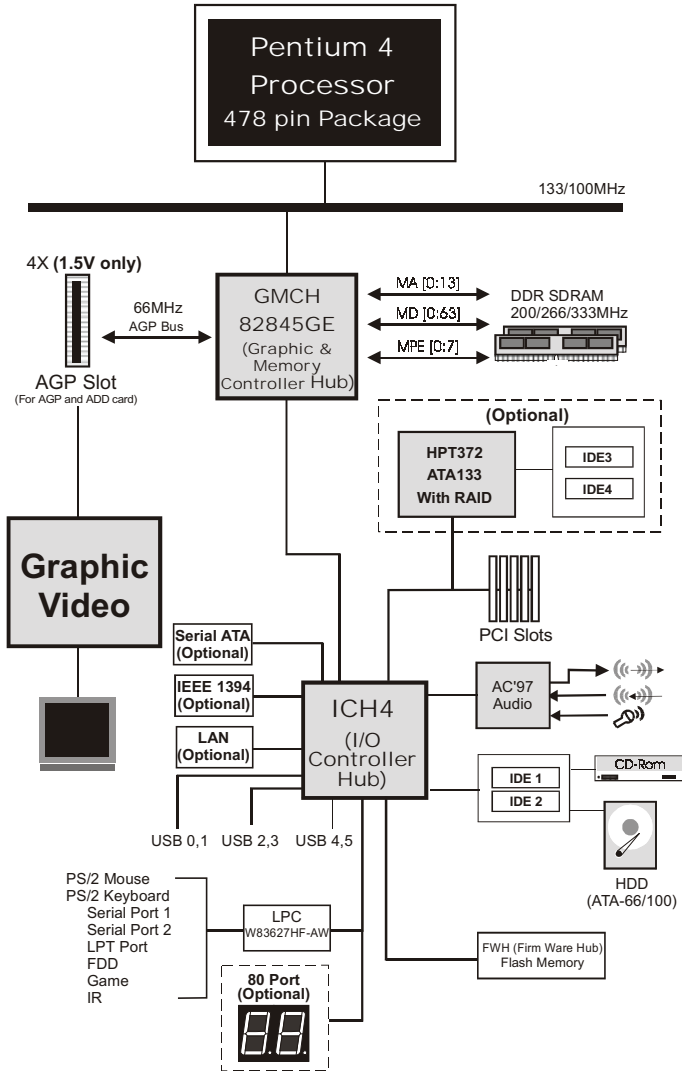
Figure 5: System Block Diagram
