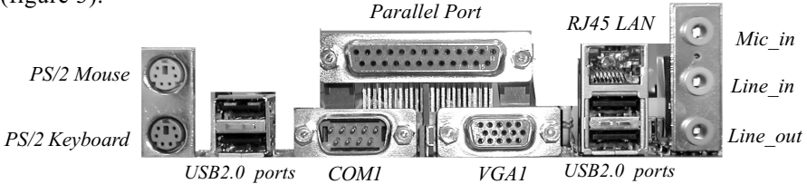
Figure 3: I/O back panel layout
