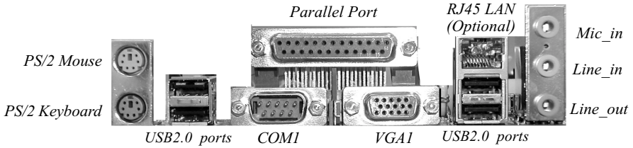
Figure 11 - I/O Ports
