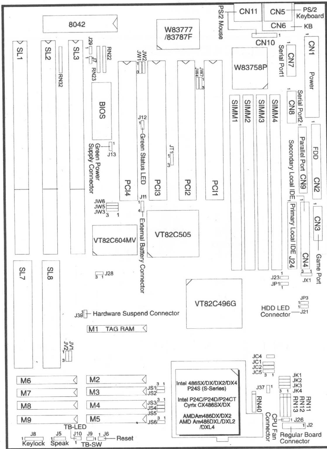
Figure 1-1. Mainboard Layout
