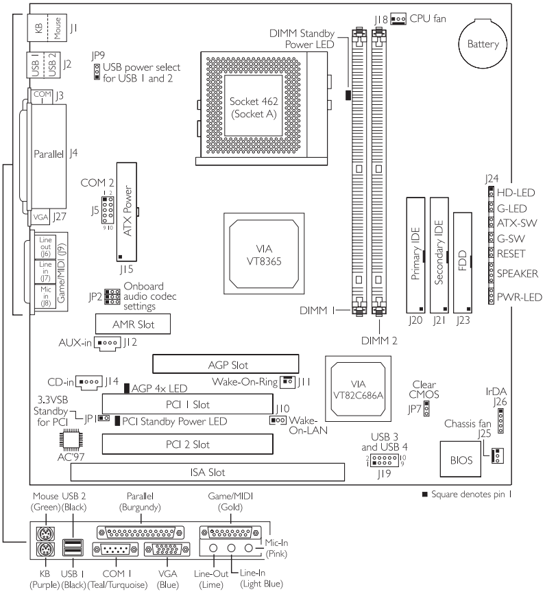
AM35-SC (VT8365 and VT82C686A)
