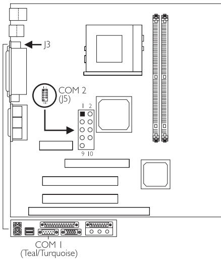
COM 1 Serial Port
