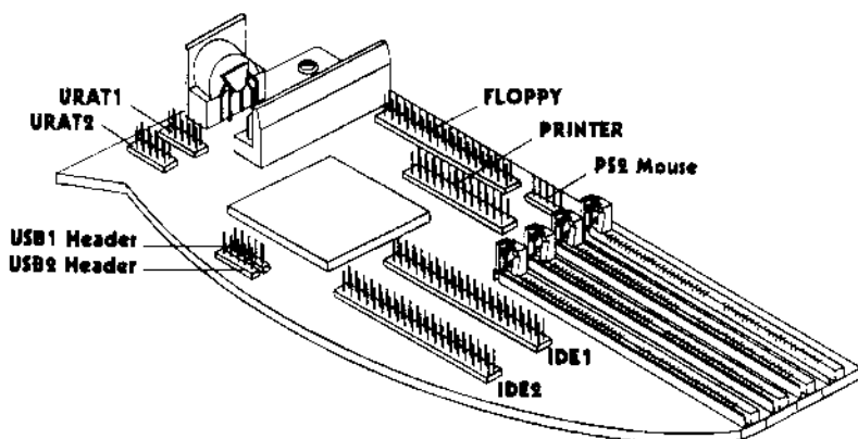
A Part of the PS1430HX-18072 Frontier II Main Board
