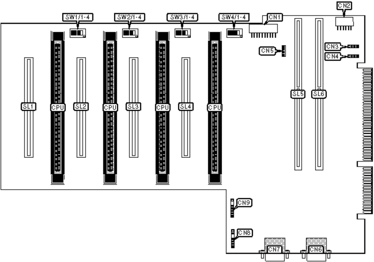
PROCESSOR BOARD
