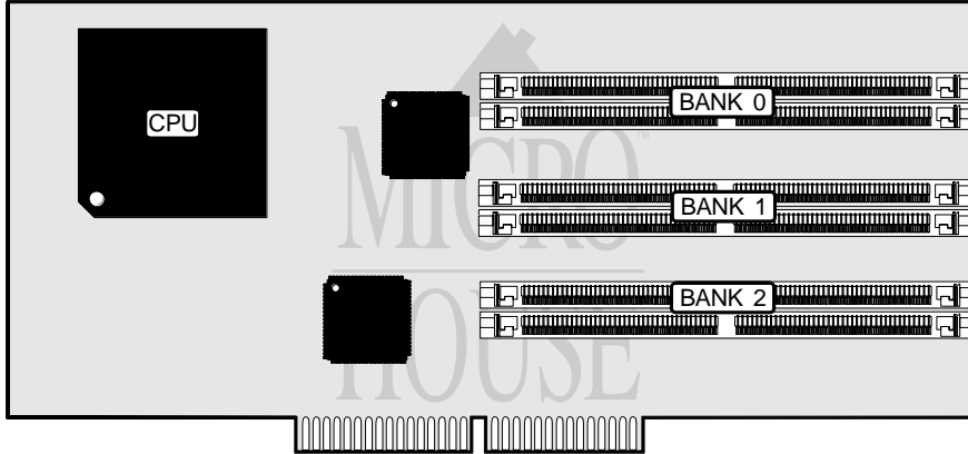
80486DX4 PROCESSOR BOARD
