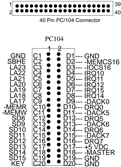
Figure PC104: 40-Pin PC/104 Connector Bus C & D
