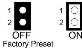
Figure 0-8 JP1: D.O.C. Memory Address Select
