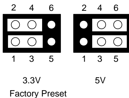
Figure 0-3 JP4: LCD Supported Voltage Select
