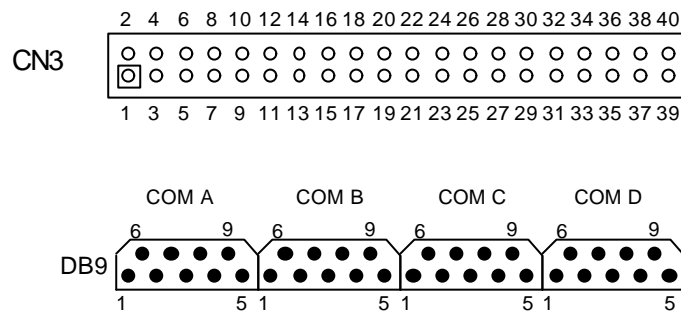
Figure 3-9 CN3: RS-232C Connector
