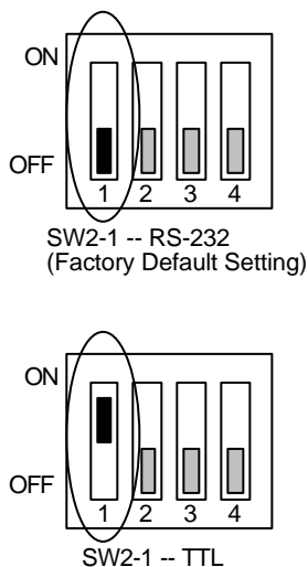
Figure 3-4 SW2-1: COM-A RS-232/TTL Select
