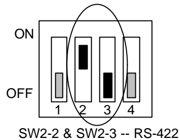
Figure 3-5 SW2-2 & SW2-3: COM-B RS-232/RS-422 Select
