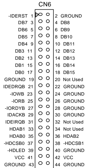
Figure 3-12 CN6: Hard Disk (IDE) Connector
