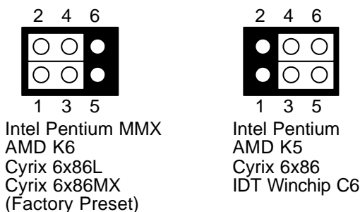
Figure 3-21 JP2: P54C/P55C CPU Type Select
