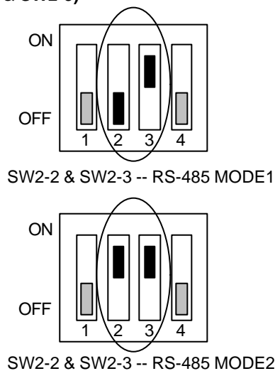
Figure 3-6 SW2-2 & SW2-3: RS-485 Mode Select
