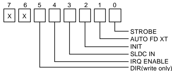
Figure 2-3 Bit' s Definition
