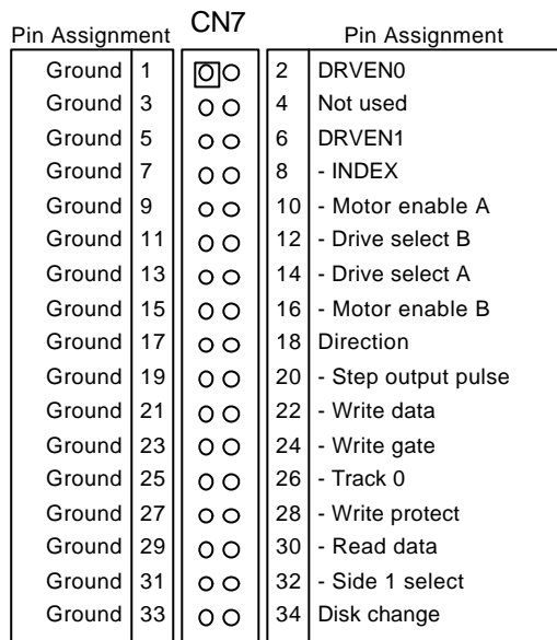
Figure 3-15 CN7: FDD Port Connector
