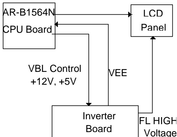
Figure 4-1 LCD Panel Block Diagram
