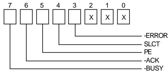
Figure 2-2 Printer Status Buffer
