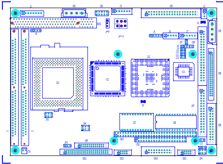
Figure 3-1 AR-B1564A Placement
