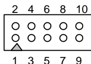
Figure 3-7 CN15: TTL Connector
