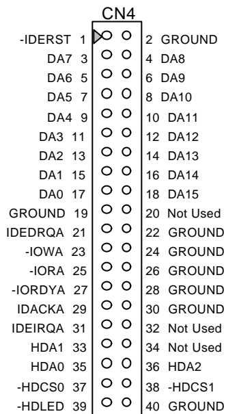
Figure 3-11 CN4: Hard Disk (IDE) Connector
