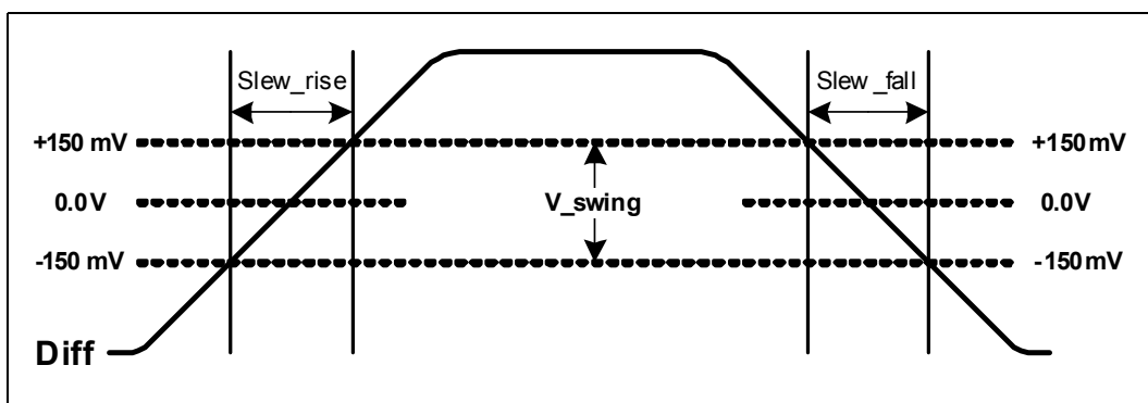
Figure 5. Differential Measurements
