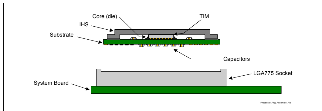
Figure 7. Processor Package Assembly Sketch
