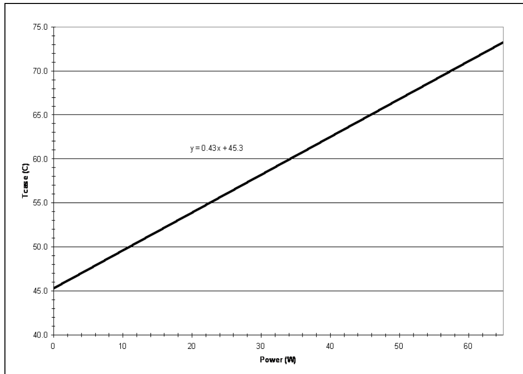
Figure 15. Thermal Profile
