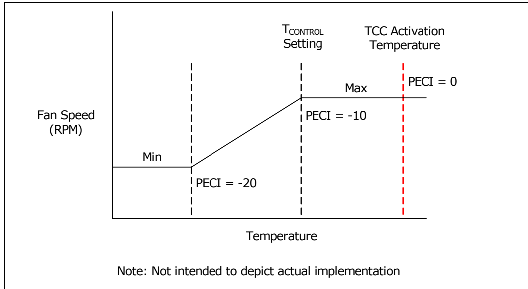
Figure 19. Conceptual Fan Control on PECI-Based Platforms
