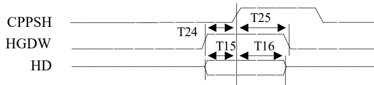
Figure 3.5 CPU Write PCI Post Write Buffer
