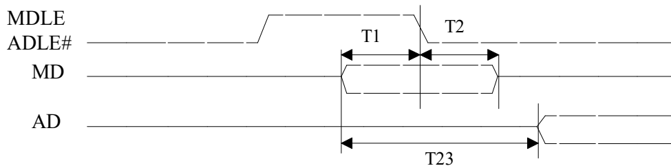
Figure 3.10 PCI Master Read DRAM
