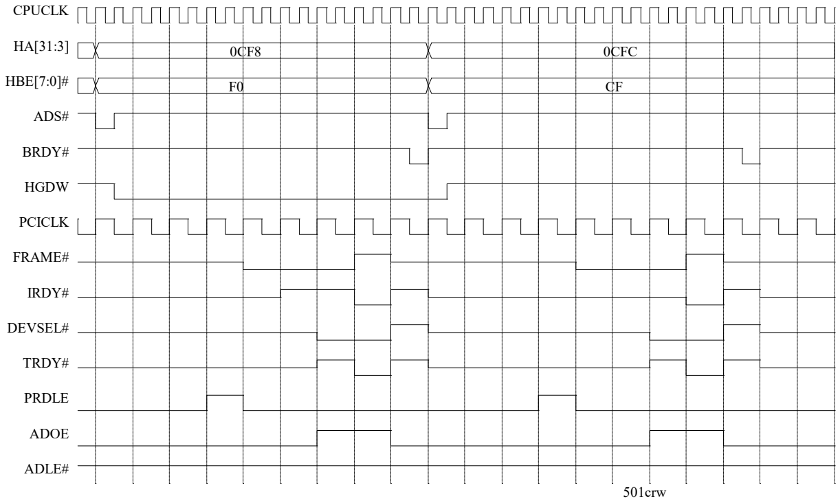
5501 Configuration Register Write Cycle
