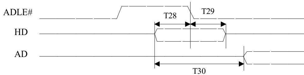
Figure 3.9 PCI Master Read Secondary Cache
