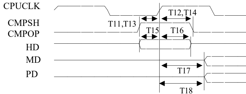
Figure 3.4 CPU Write DRAM Cycle
