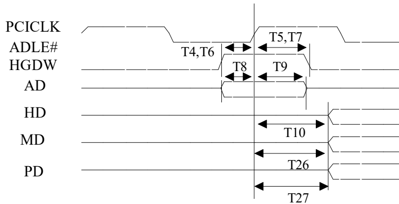
Figure 3.8 CPU Read PCI Slave Cycle
