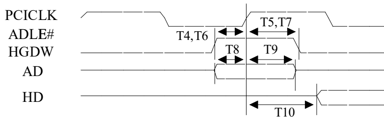
Figure 3.3 CPU Read PCI Slave Cycle
