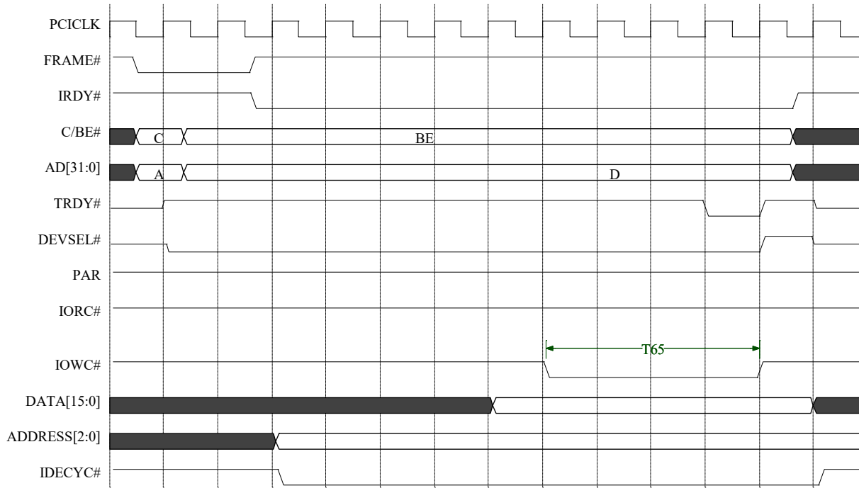
Figure 4.14 IDE Basic Write Cycle (One Word)
