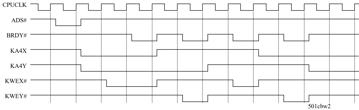
Cache Burst Write Hit Cycle 4-2-2-2
