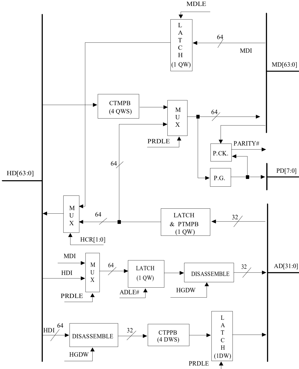
Figure 3.1 PLDB Block Diagram
