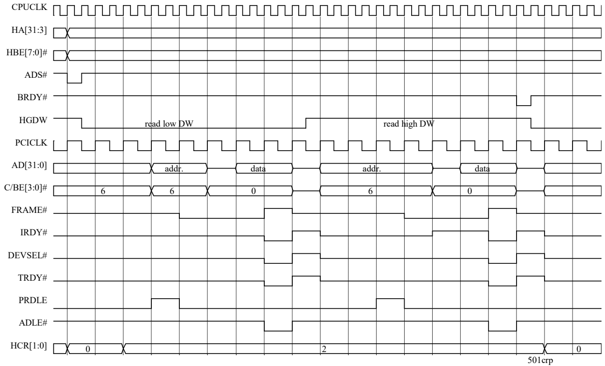
CPU Read PCI Slave
