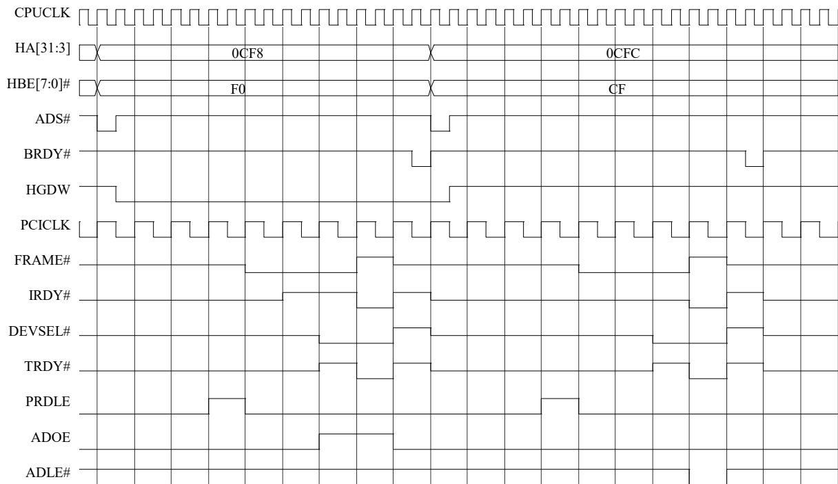
5501 Configuration Register Read Cycle
