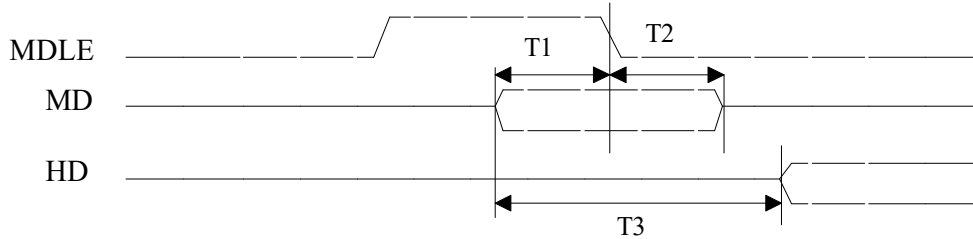
Figure 3.2 CPU Read DRAM Cycle
