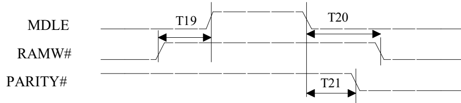
Figure 3.7 PARITY# Generation Reading DRAM Cycle
