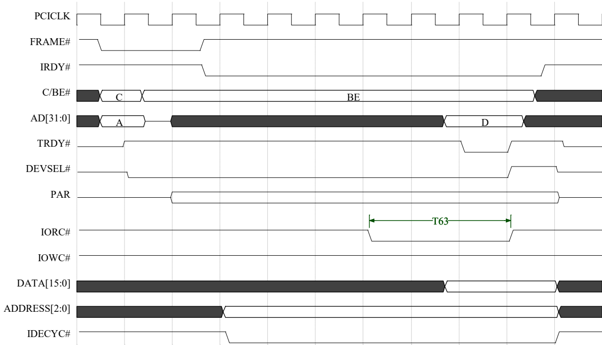
Figure 4.16 IDE Basic Read Cycle (One Word)
