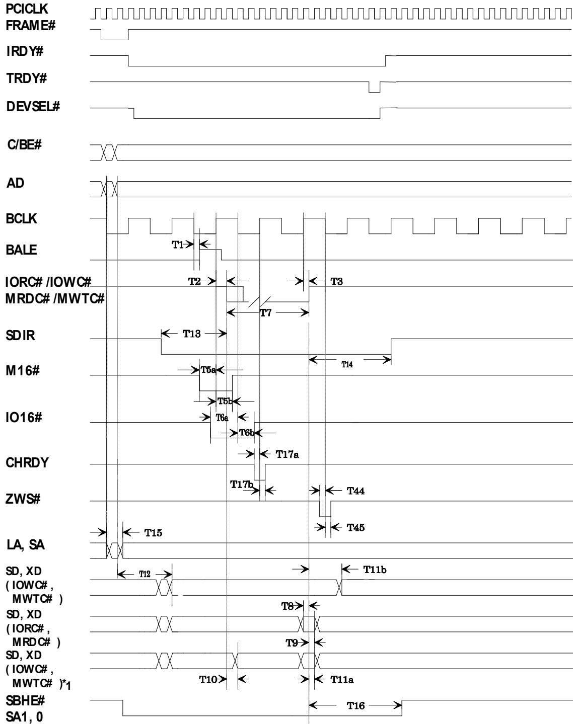
Figure 4.2 PCI to AT Bus Cycle
