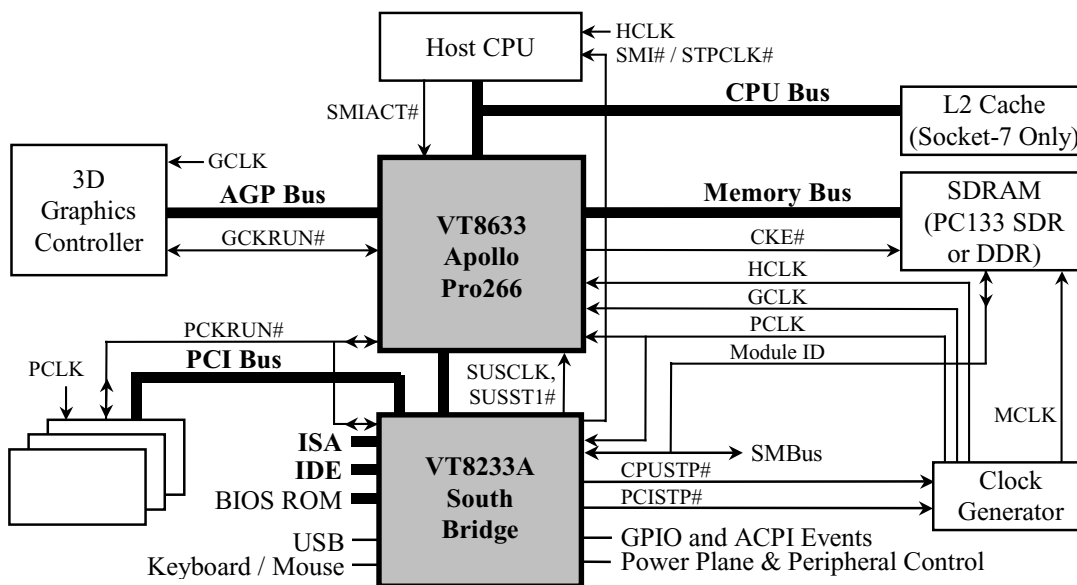
Figure 4. System Block Diagram Using the VT8633 North Bridge
