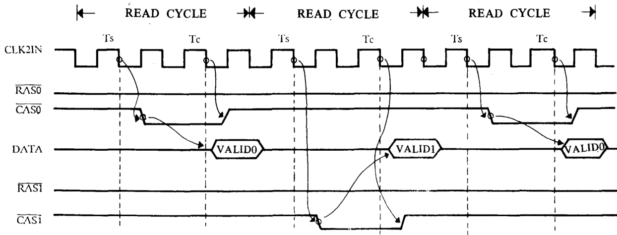
Figure 2.2 Page-Interleaved Mode Operation (Read Cycle)
