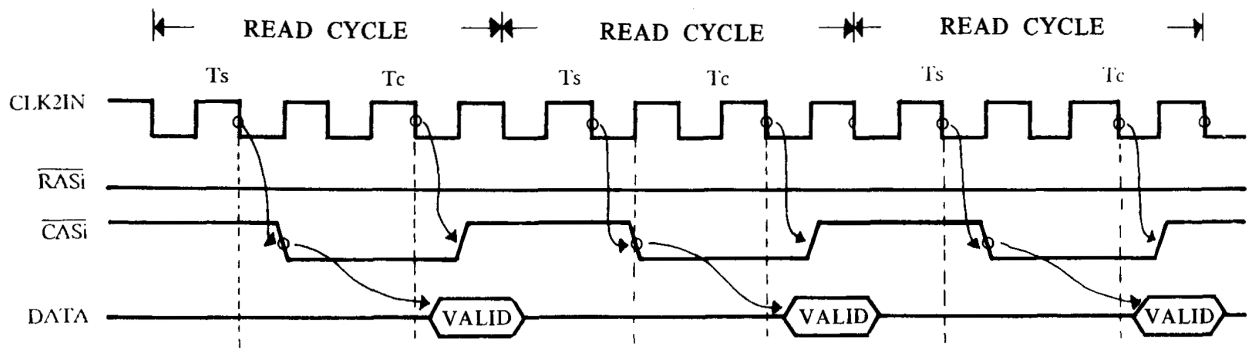
Figure 2.1 Page Mode Operation (Read Cycle)
